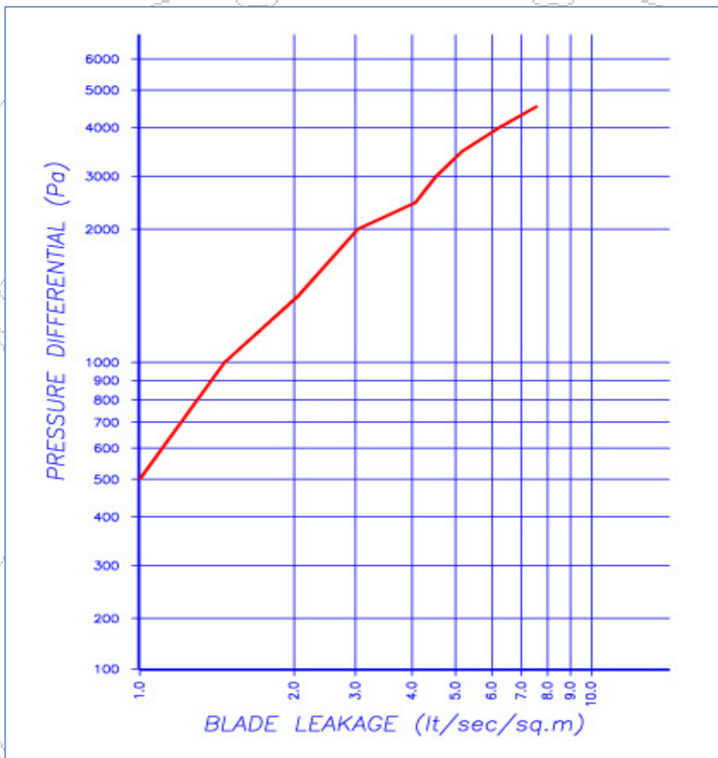
Graph of air leakage vs. pressure differential through closed blades
